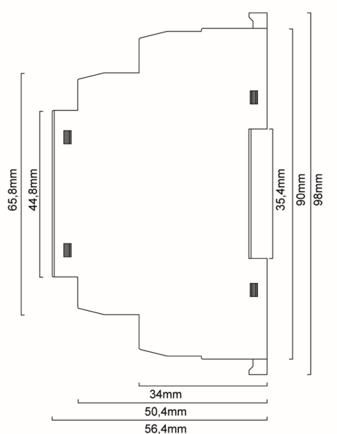
Geometrie 4x RM16 I HS
