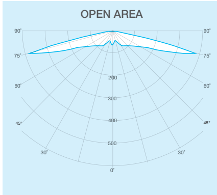
Photometric details
