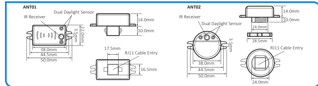
ANT01: Mounting hole size 21 x 17mm (L x W)
