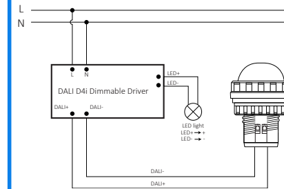
DALI D4i Driver (Integrated DALI BUS power supply)
