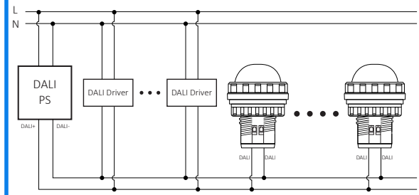
DALI System (DALI BUS power supply)
